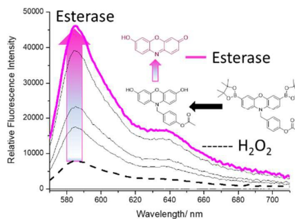
Fig. 6 - Fluorescence spectra of Pinkment-OAc (0.5 \mu\text{M} ) following incubation (15 mins) with PLE (0.1 - 0.6 U) and subsequent addition of H 2 O 2 (1 mM). The dotted line represents the response to hydrogen peroxide on its own. The data was collected in PBS buffer (100% w/w H 2 O) at pH=7.4 ,25 ^\circ\text{C} . \lambda_{\text{ex}} =545-20 nm Dashed line represents H 2 O 2 (1 mM) addition only
