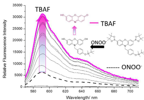
Fig. 4 - Fluorescence spectra of Pinkment-OTBS (5 \mu\text{M} ) with the addition of \text{ONOO}^- (20 \mu\text{M} ) followed by incremental additions of TBAF (0 – 10 mM) measurements were taken after 90 mins of both additions. The data was obtained in PBS (52% w/w MeOH:H 2 O), pH = 8.2 at 25 ^\circ\text{C} . \lambda_{\text{ex}} =545-20 nm. Dashed line represents \text{ONOO}^- (20 \mu\text{M} ) addition only
