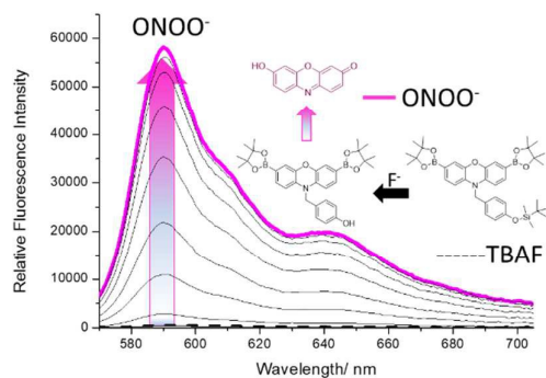
Fig. 3 – Fluorescence spectra of Pinkment-OTBS (5 \mu\text{M} ) with addition of TBAF (10 mM) and incubated for 1 h and then measured. Followed by incremental additions of \text{ONOO}^- (0 – 20 \mu\text{M} ) The data was obtained in PBS (52% w/w MeOH:H 2 O), pH = 8.2 at 25 ^\circ\text{C} . \lambda_{\text{ex}} =545-20 nm.
