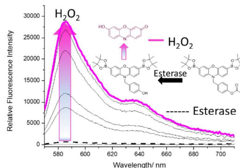
Fig. 5 - Fluorescence spectra of Pinkment-OAc (5 \mu\text{M} ) for the incubation (15 min) of porcine liver esterase, PLE (0.6 U) followed by incremental additions of H 2 O 2 (0 – 1 mM) measurements were taken after 1 h. The data was collected in PBS (100% w/w H 2 O) at pH=7.4 ,25 ^\circ\text{C} . \lambda_{\text{ex}} =545-20 nm.
