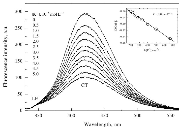
Figure 2 Fluorescence spectra of PTDMAB in 80% \text{H}_2\text{O} -dioxane mixture in the presence of K^+ . Inset is the double reciprocal plot for the binding of K^+ to PTDMAB aggregates.
