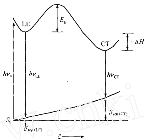
Scheme 2. Potential curves for the states involved in the CT process.
