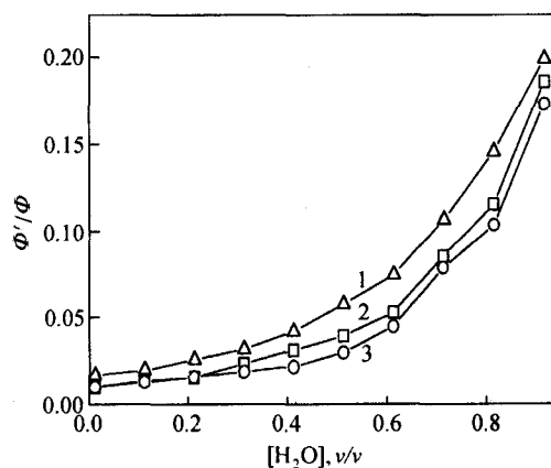
Fig. 6. Variations of \Phi'/\Phi of SDMAS with water content by volume in water-organic solvent mixtures. Organic solvents are ethanol (EtOH, 1), acetonitrile (ACN, 2), and 1, 4-dioxane (DiOX, 3), respectively.
