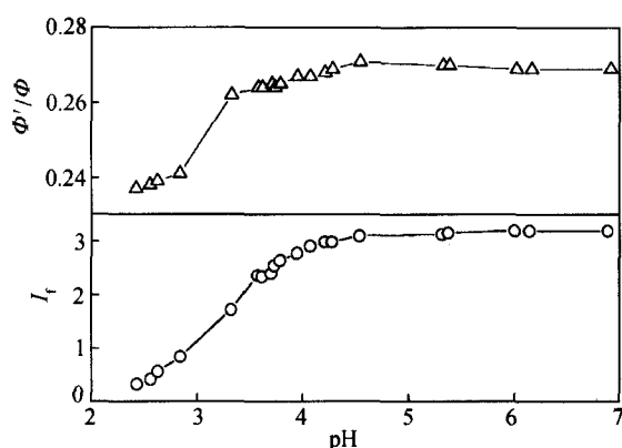
Fig. 4. pH dependence of \Phi'/\Phi ratio and total fluorescence intensity ( I_t ) of SDMAS in aqueous solution. pH was tuned by NaOH or HCl.
