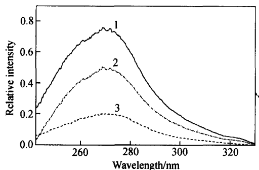
Fig. 2. Fluorescence excitation spectra and absorption spectrum of SDMAS in water. Curves represent: 1, excitation spectrum with \lambda_{em}=364 nm; 2, absorption spectrum with \lg\epsilon_{270nm}=4.34 ; 3, excitation spectrum at \lambda_{em}=470 nm, respectively.
